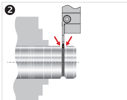
2. Chamfering
