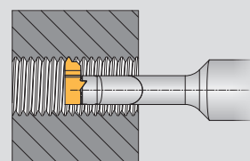
Holder and inserts in left hand version
