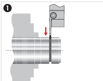
1. Pre-grooving
