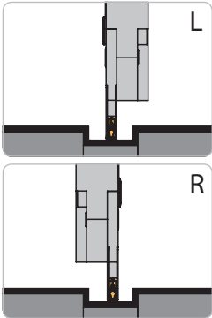
Left holder and left module mounted. Height-adjustable holder. W=W-notch
